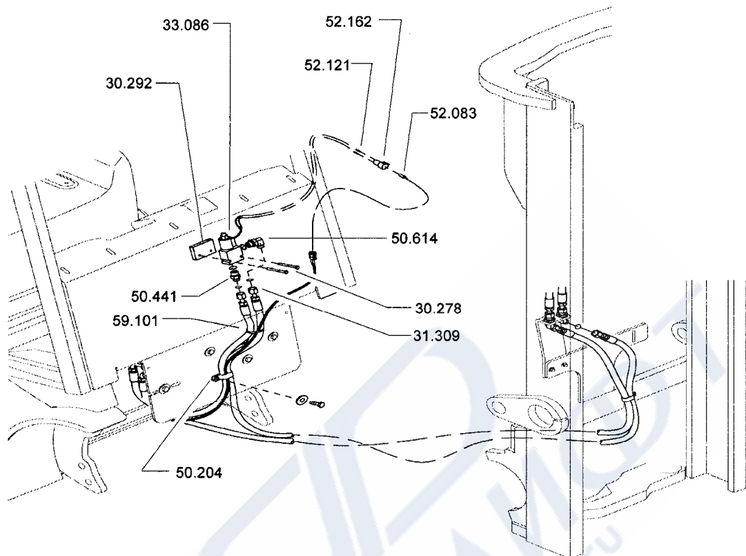
AUXILIARY VALVE INSTALLATION
