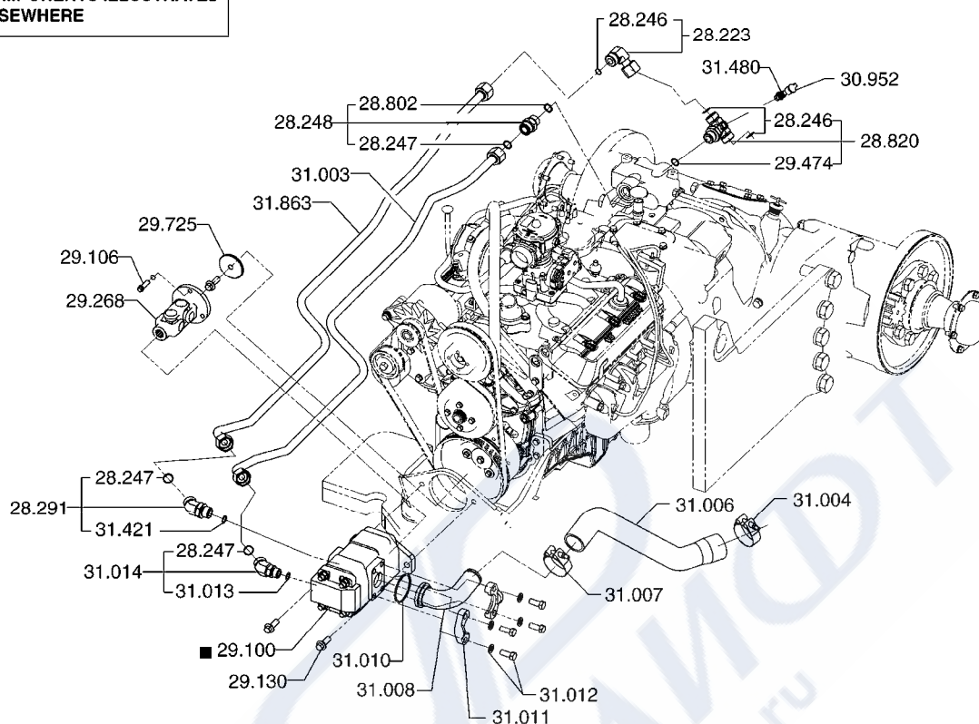
HYDRAULIC PUMP MOUNTING
