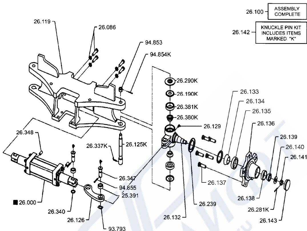
STEERING AXLE
