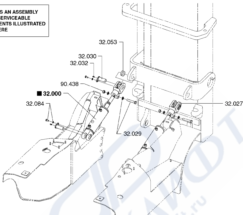
TILT CYLINDER MOUNTING
