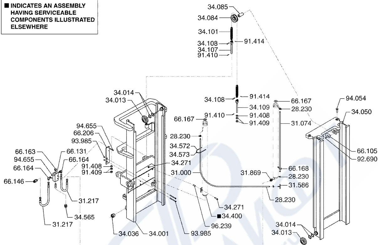
STANDARD UPRIGHT
