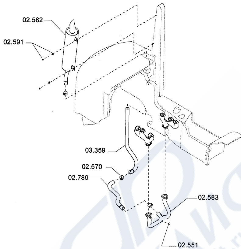
EXHAUST SYSTEM
