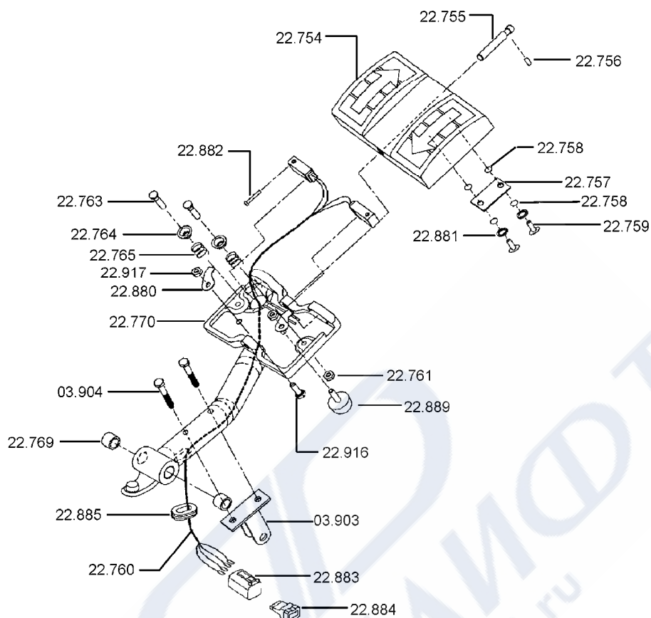
UNITROL PEDAL INSTALLATION
