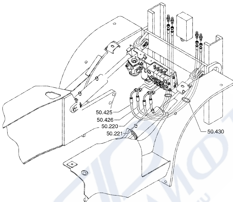
AUX VALVE PLUMBING
