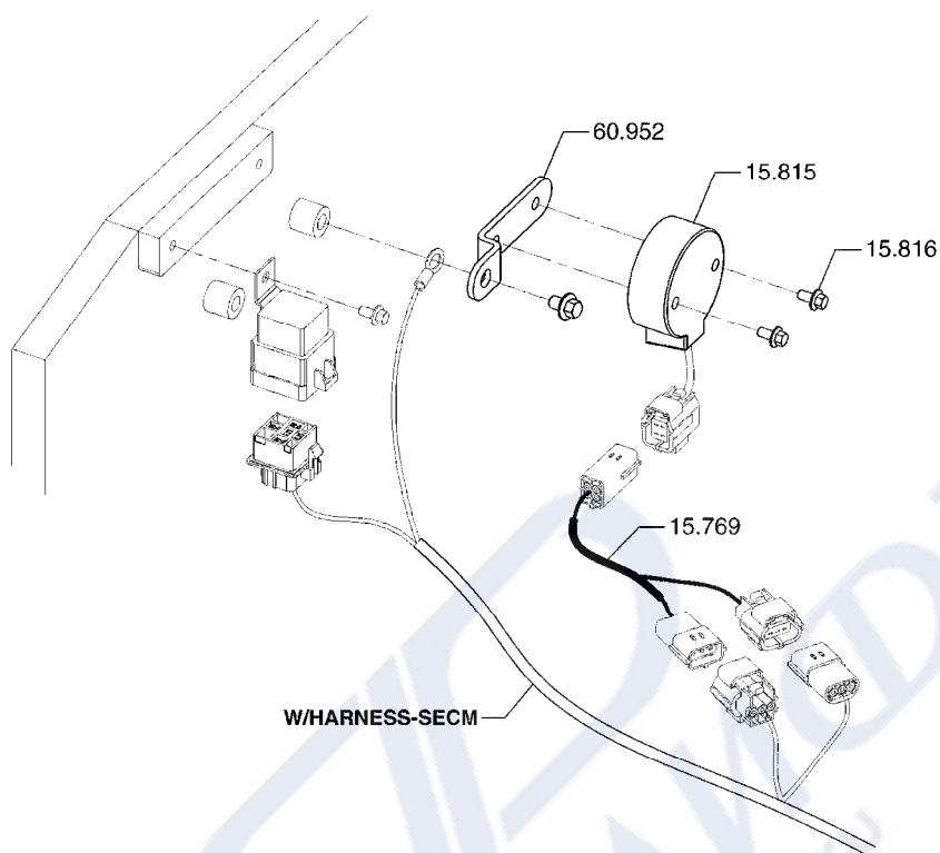
DELAY TIMER MOUNTING
