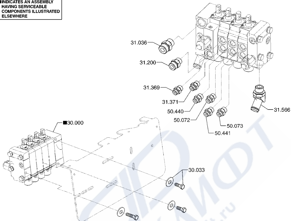
HYDRAULIC VALVE INSTALLATION
