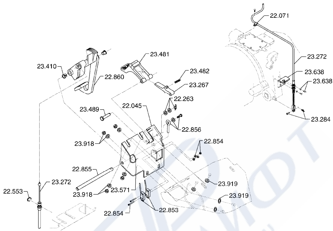
PARKING BRAKE LINKAGE
