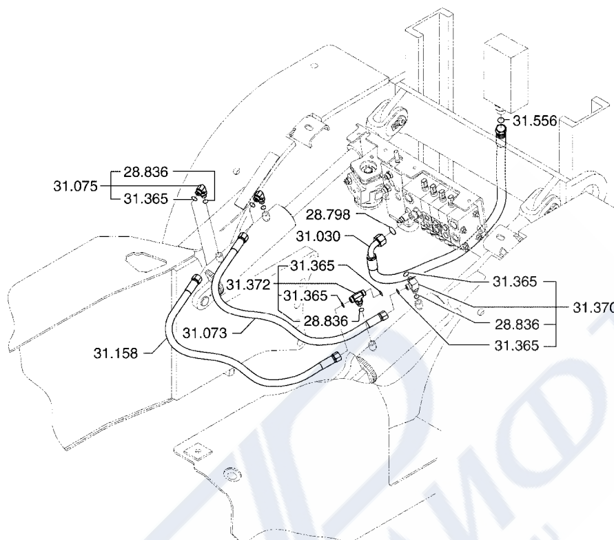
LIFT/TILT PLUMBING
