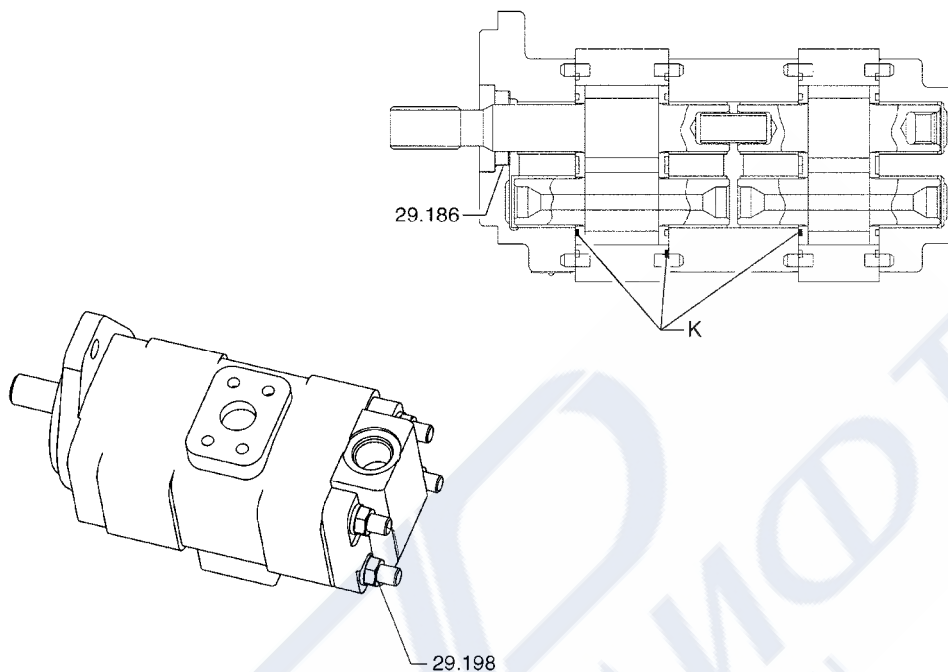
HYDRAULIC PUMP ASSEMBLY
