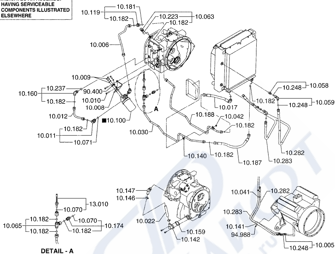
TRANS COOLING LINES
