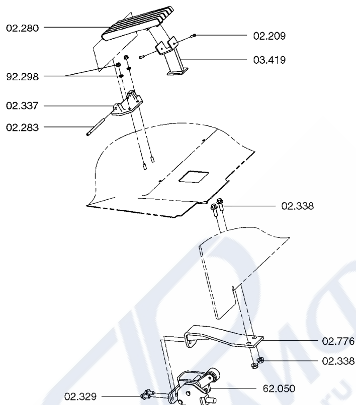
ACCELERATOR PEDAL & LINKAGE
