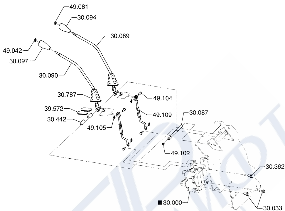
MAIN CONTROL VALVE 2-SPOOL
