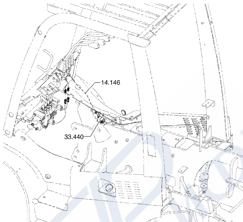
SOLENOID VALVE ELECTRIC MOUNTING
