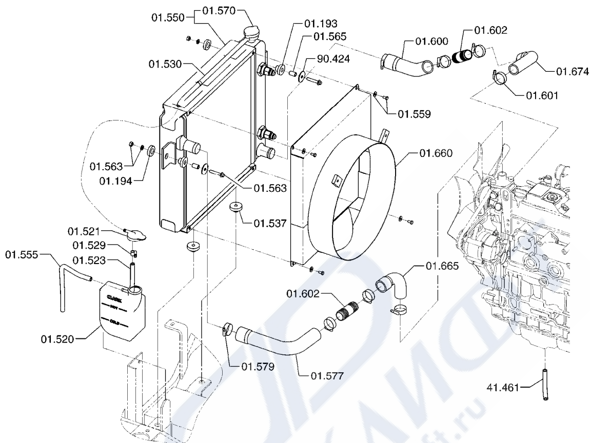
COOLING SYSTEM
