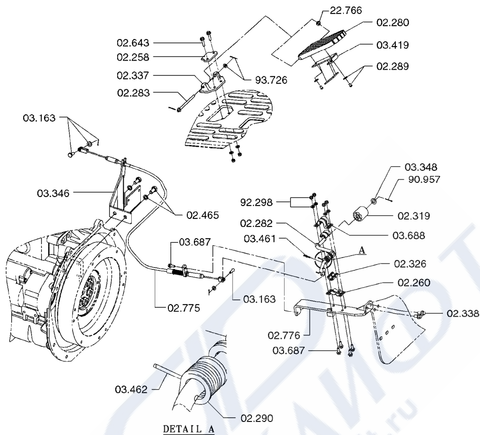
ACCELERATOR LINKAGE
