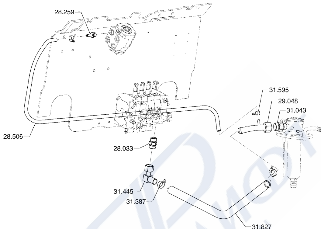
HYDRAULIC RETURN LINES
