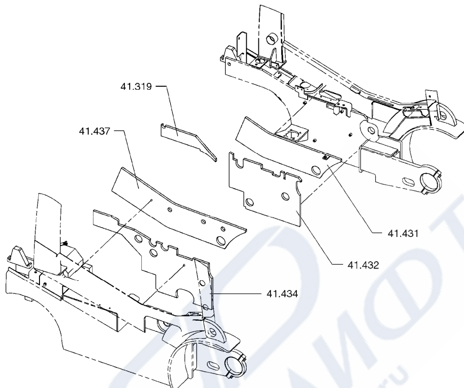
SPONGE MOUNTING
